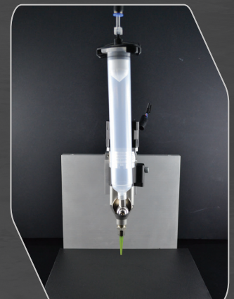
Extrusion (Robocasting)
